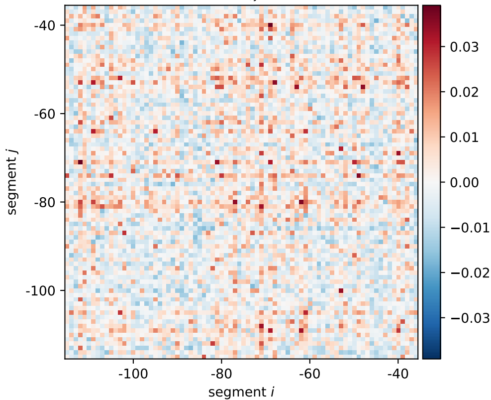
yjiY expression shift \xi_{i,j}[0101, 0110, 1010]
