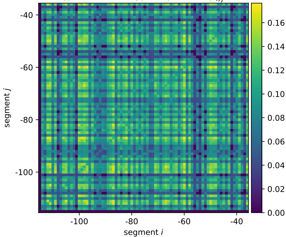
yjiY mean wildtype expression \mu_{i,j}^*
