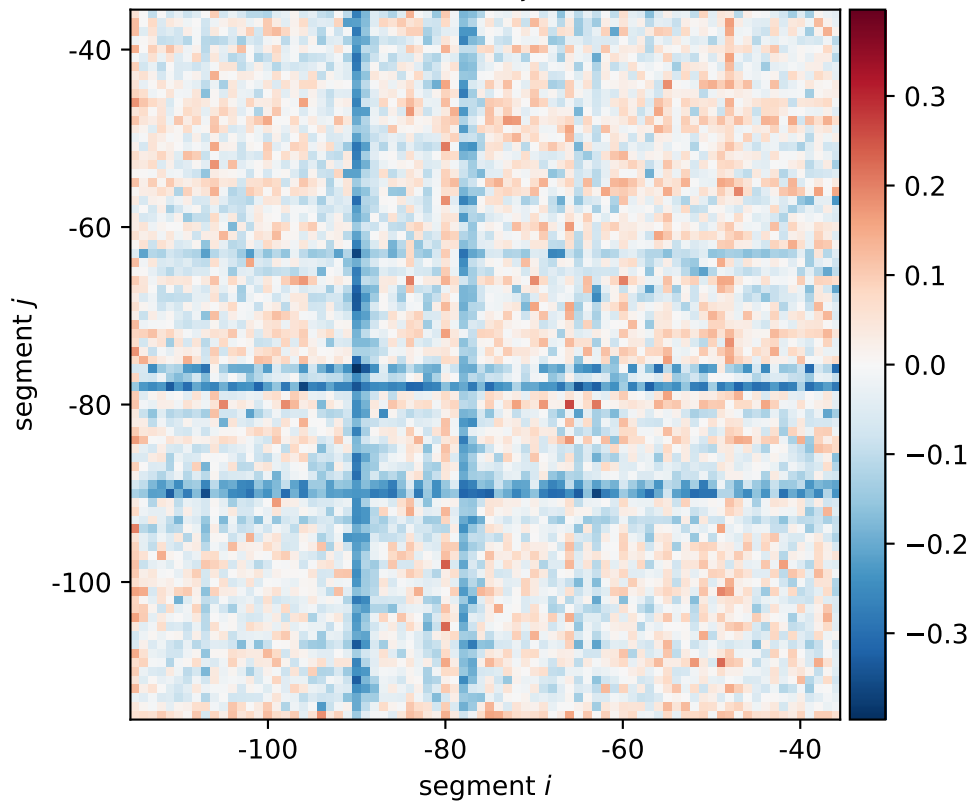
ykgE expression shift \xi_{i,j}[0101, 0110, 1010]
