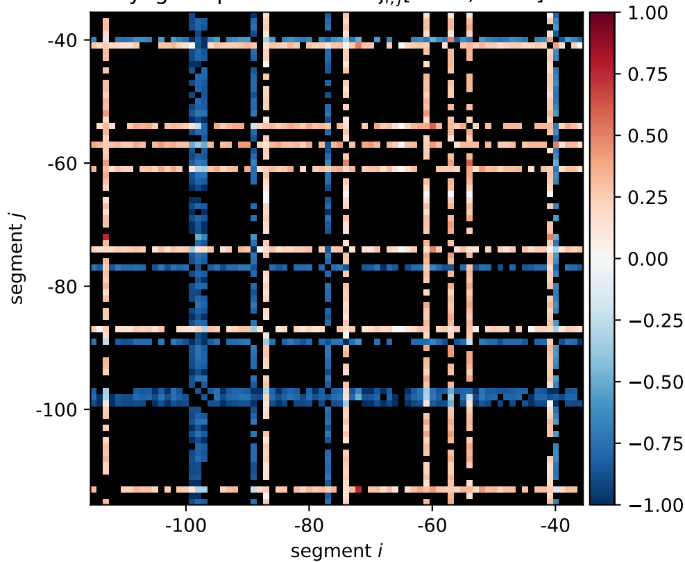
ykgE expression shift \xi_{i,j}[0011, 1100]
