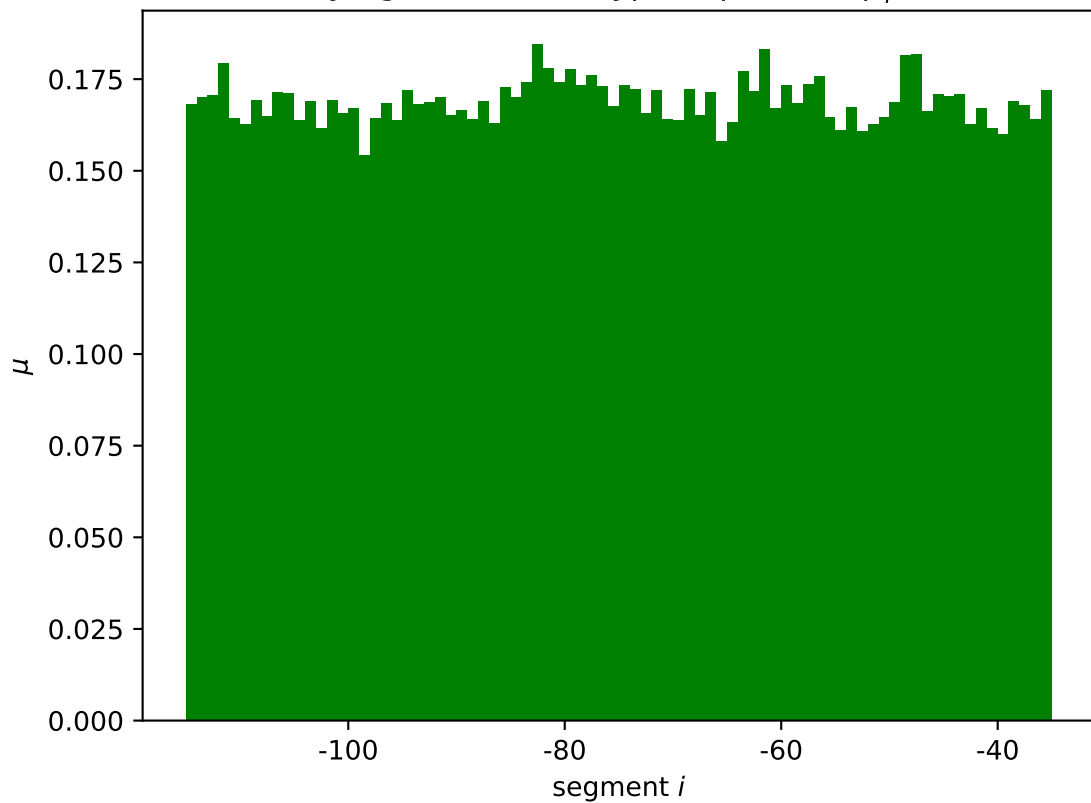
ymgG mean wildtype expression \mu_i^*
