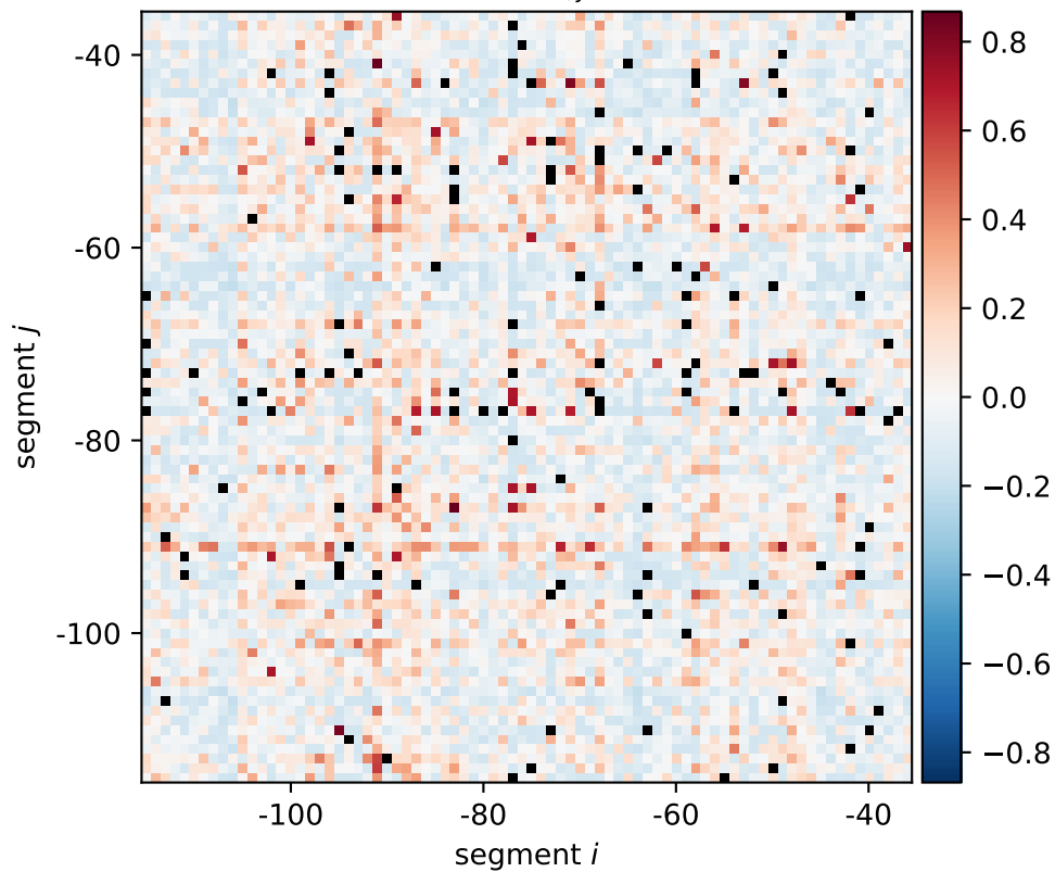
ymgG expression shift \xi_{i,j}[0101, 0110, 1010]
