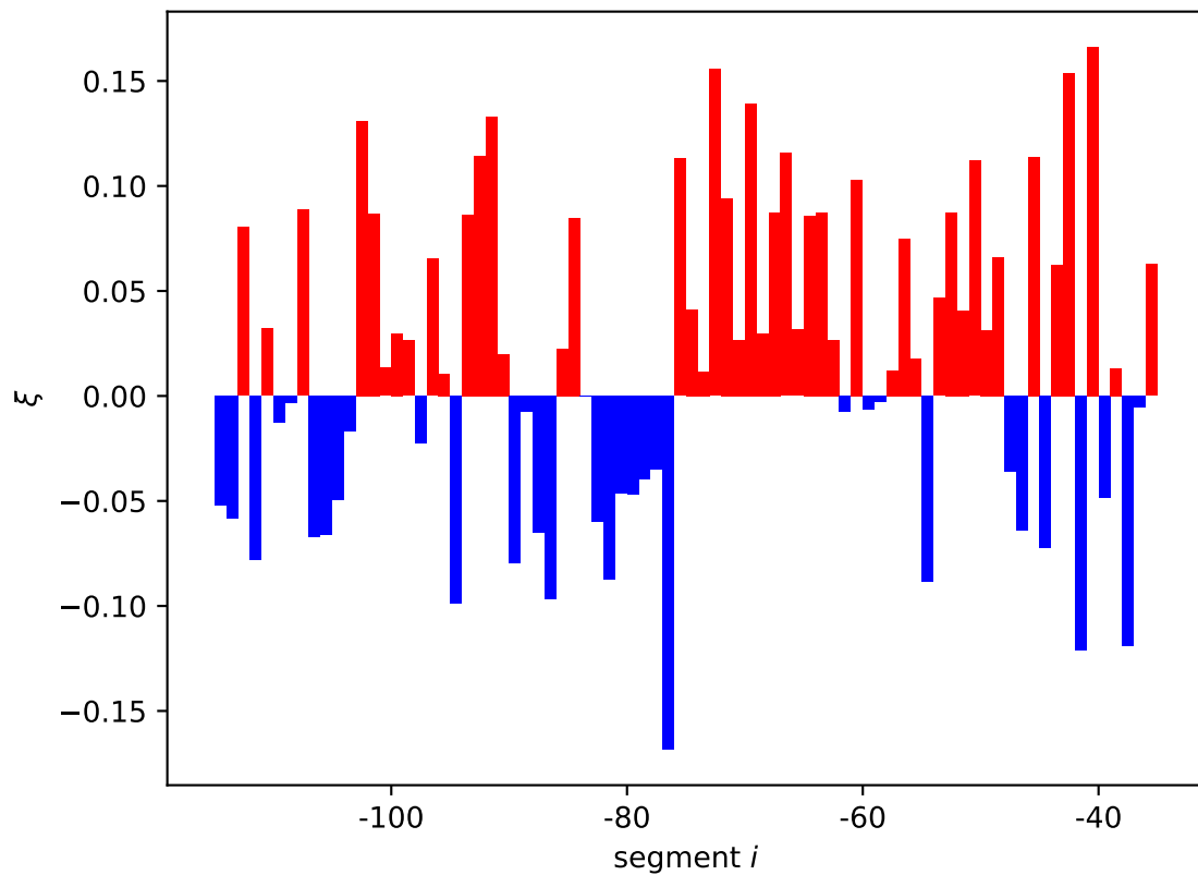
ymgG expression shift \xi_i[01, 10]
