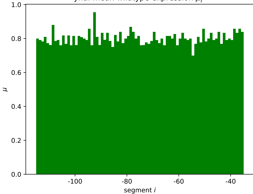
ynal mean wildtype expression \mu_i^*
