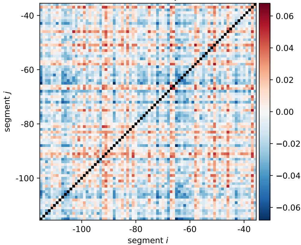
yncD expression shift \xi_{i,j}[\text{0011}, \text{1100}]
