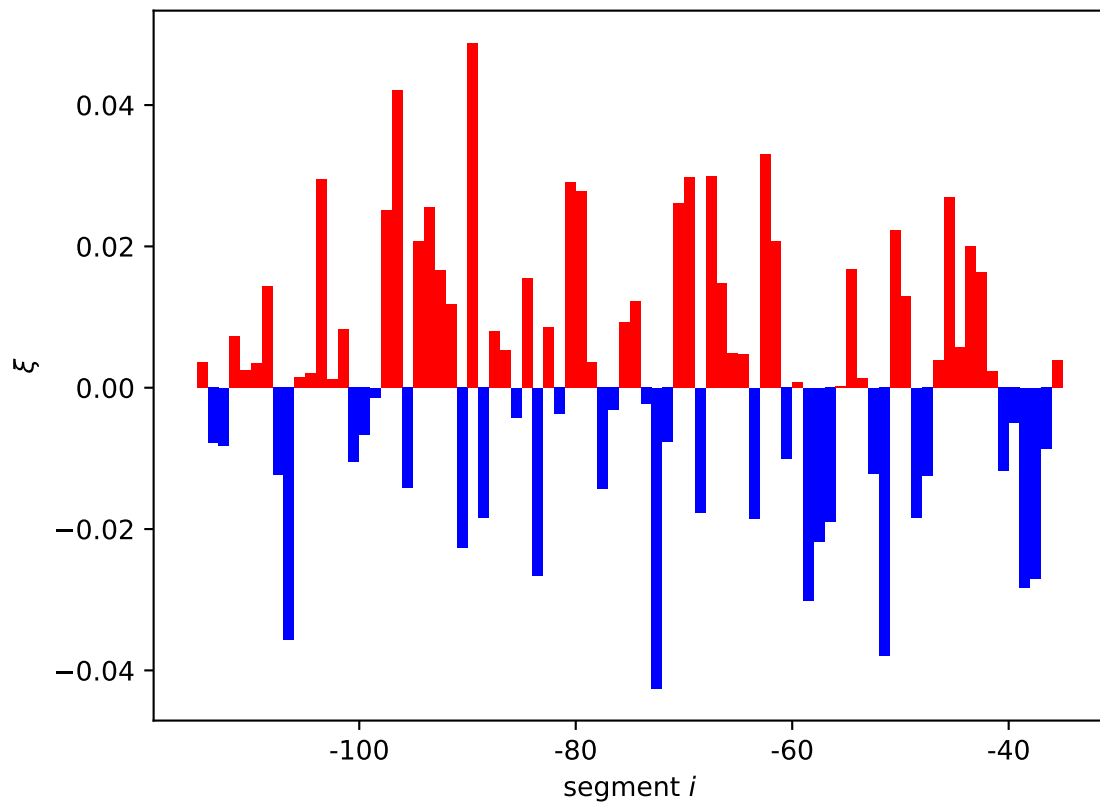
yncD expression shift \xi_i[01, 10]
