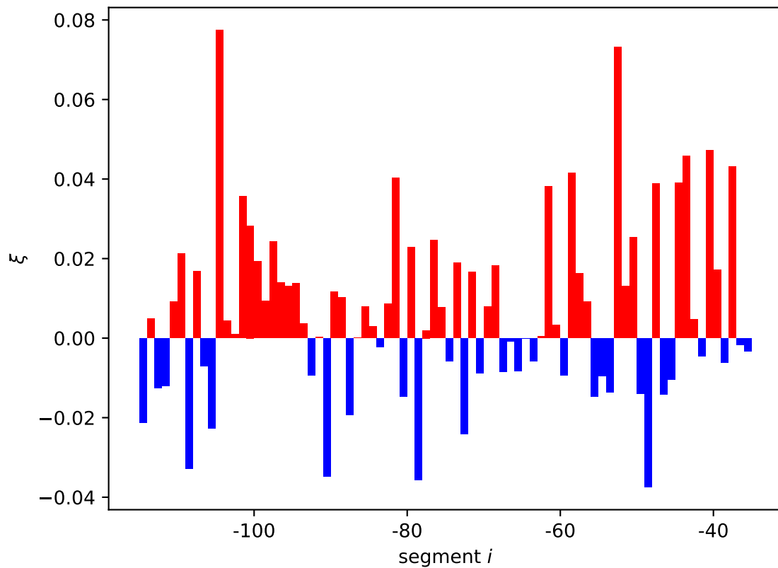
yqhC expression shift \xi_i[01, 10]
