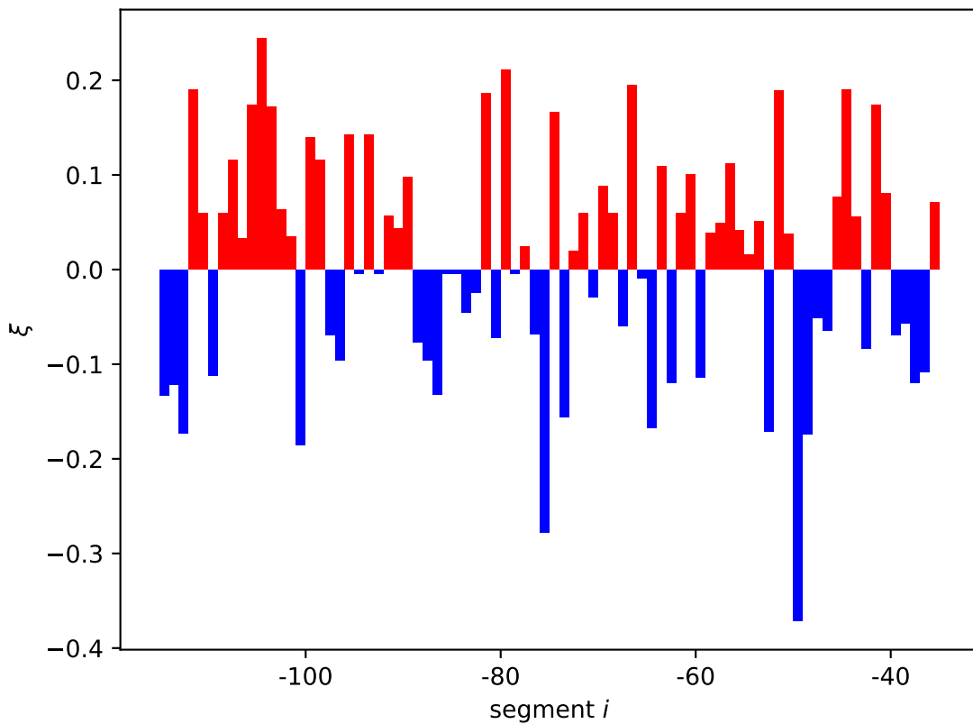
yqhC expression shift \xi_i[01, 10]
