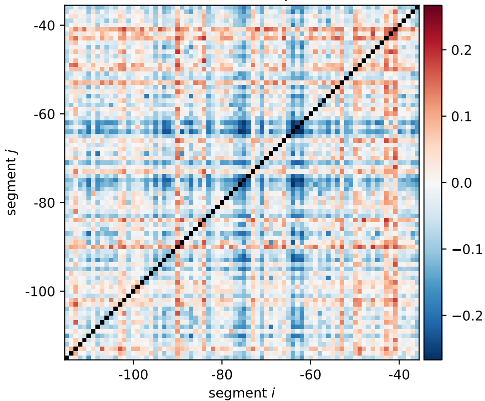
zapB expression shift \xi_{i,j}[\text{0011}, \text{1100}]
