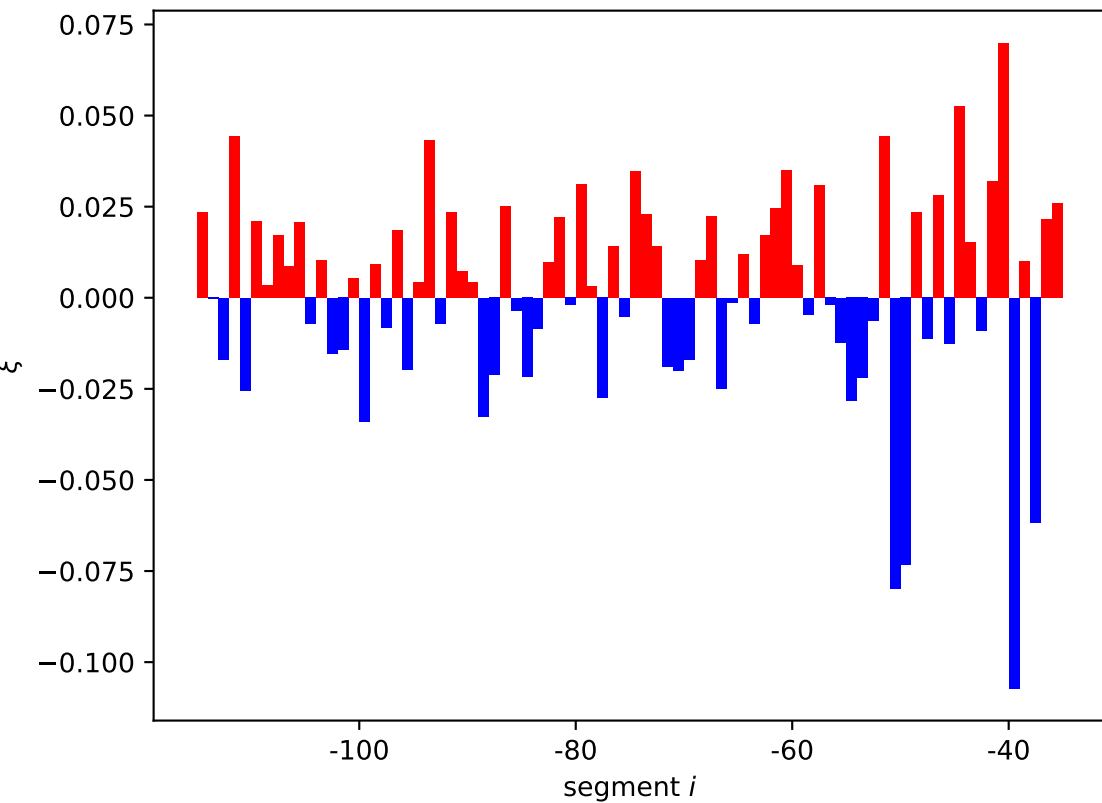
znuA expression shift \xi_i[01, 10]
