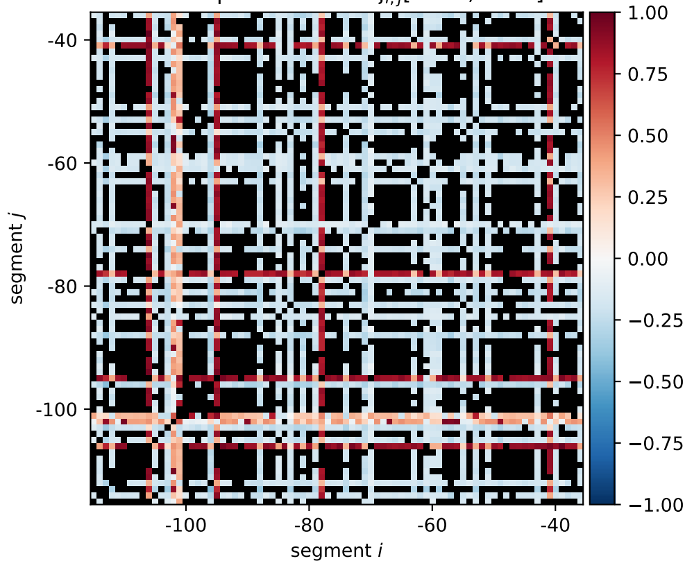
znuA expression shift \xi_{i,j}[\text{0011}, \text{1100}]
