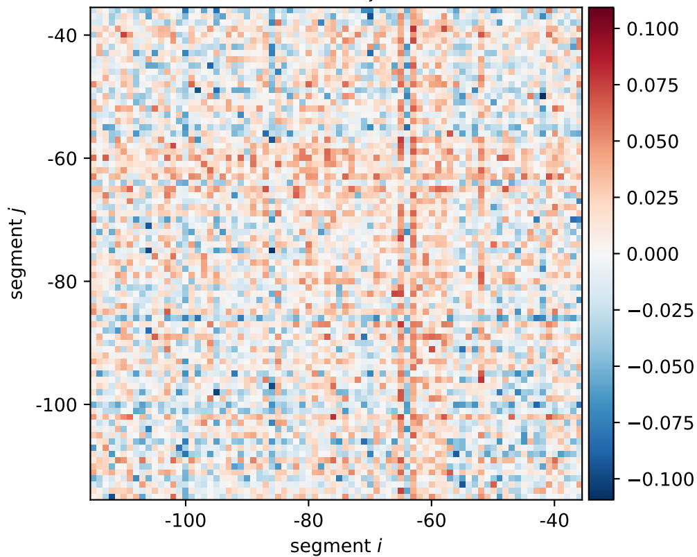
znuCB expression shift \xi_{i,j}[0101, 0110, 1010]
