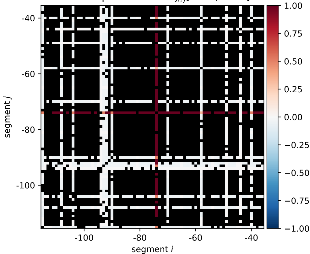
znuCB expression shift \xi_{i,j}[0011, 1100]
