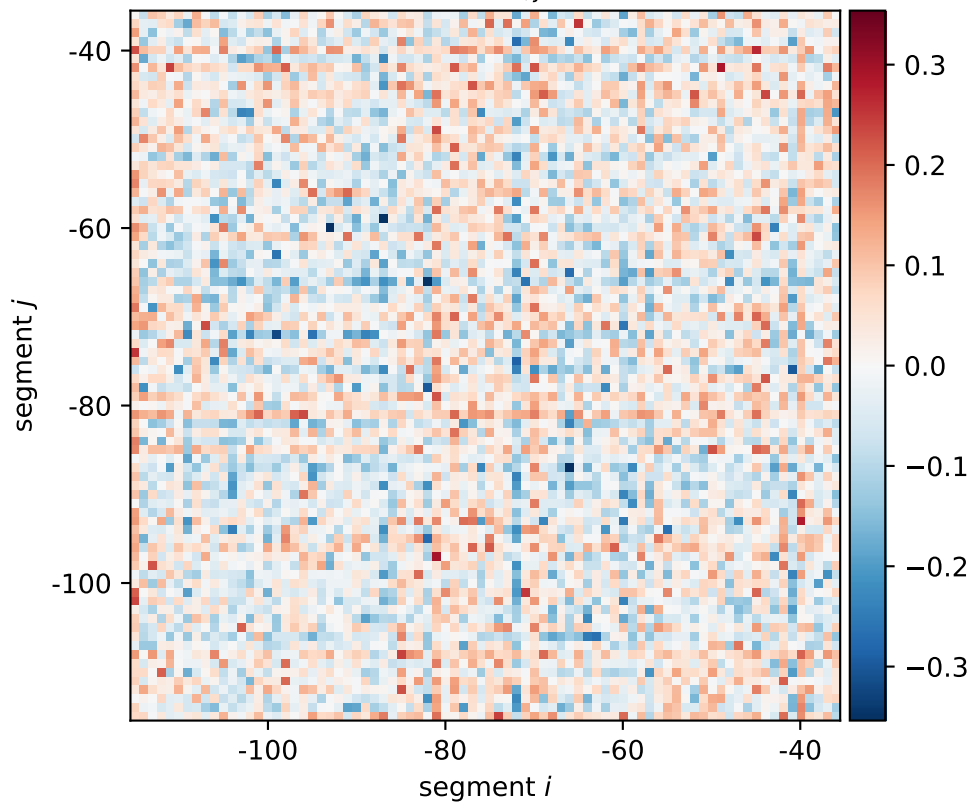
znuCB expression shift \xi_{i,j}[\text{0101}, \text{0110}, \text{1010}]
