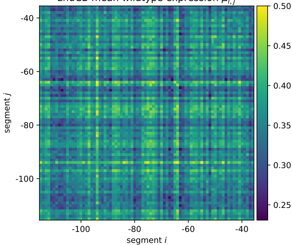
znuCB mean wildtype expression \mu_{i,j}^*
