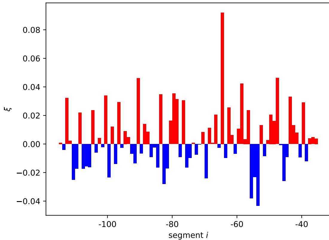
zupT expression shift \xi_i[01, 10]
