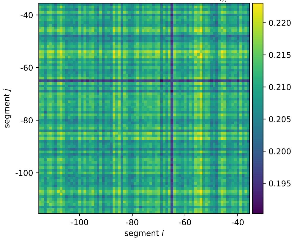
zupT mean wildtype expression \mu_{i,j}^*
