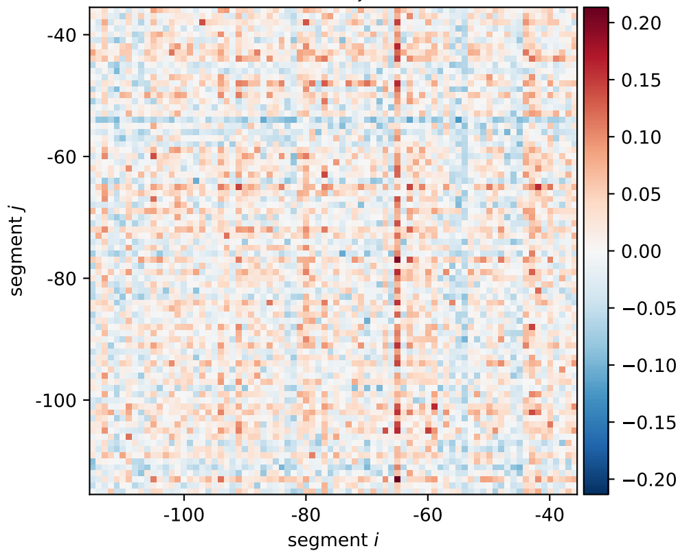
zupT expression shift \xi_{i,j}[0101, 0110, 1010]
