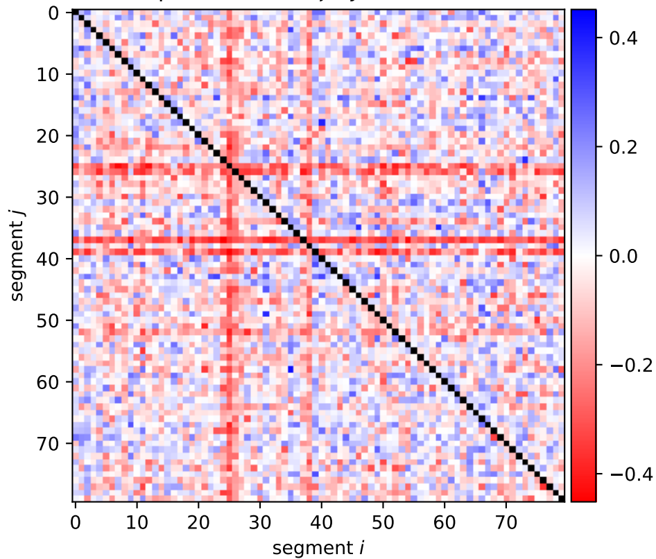
Expression shift \xi[i, j; (0, 1), (1, 0)]
