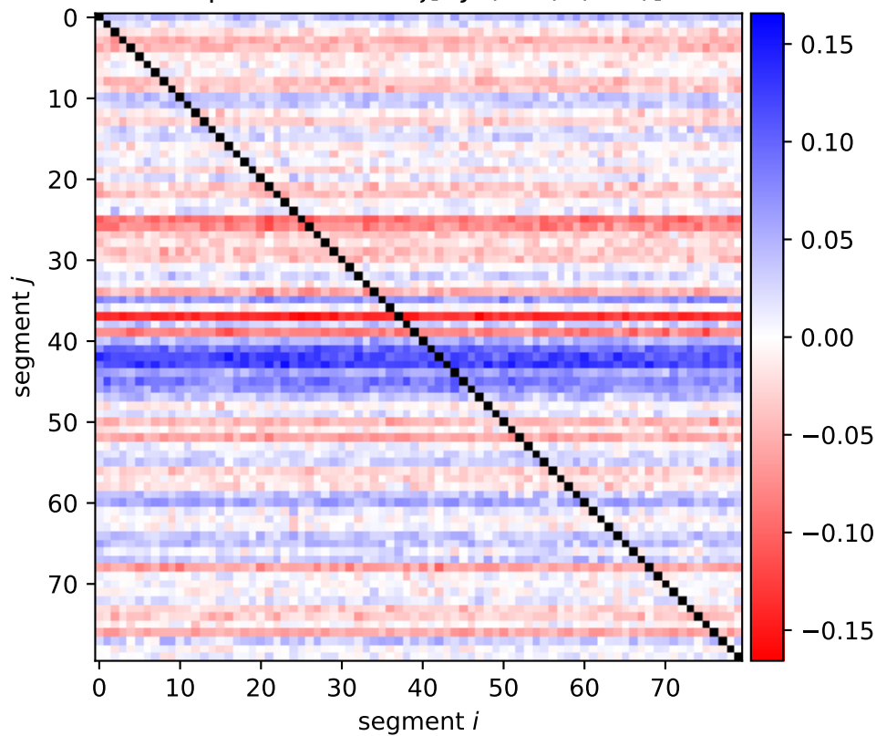
Expression shift \xi[i, j; (0, 0), (1, 0)]
