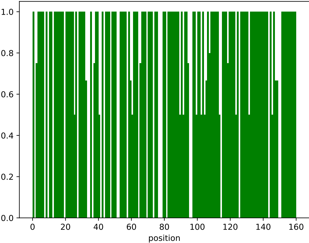
\mu_i[1] (singlets)
