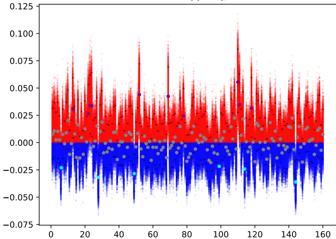
Bootstrapped \xi_i
