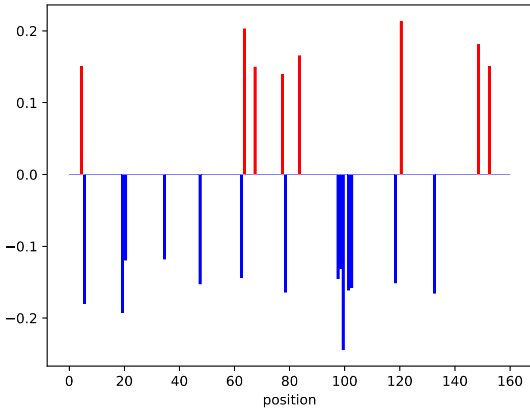
Boostrapped \xi
