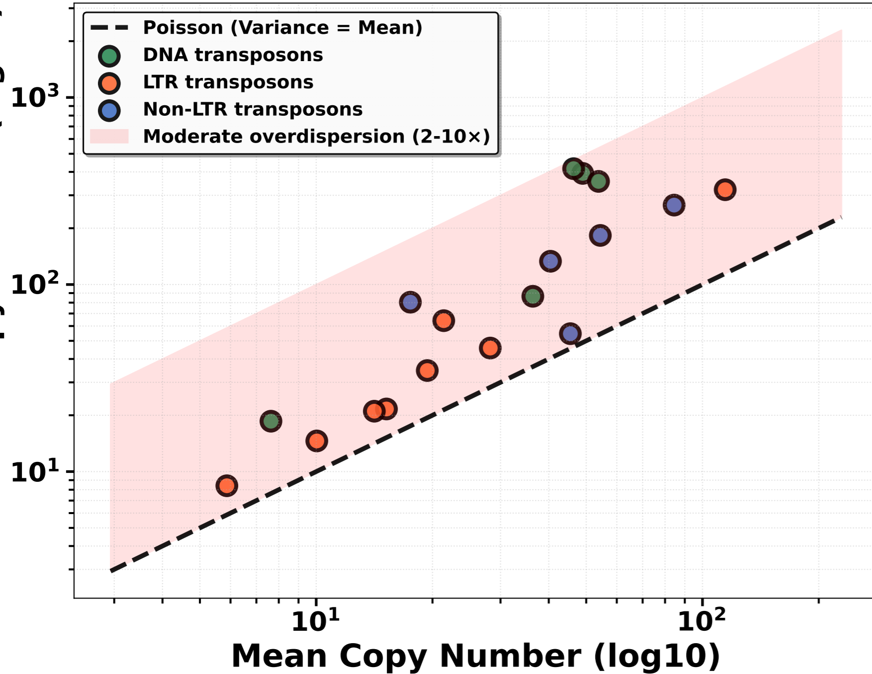
Variance/Mean (log10)
