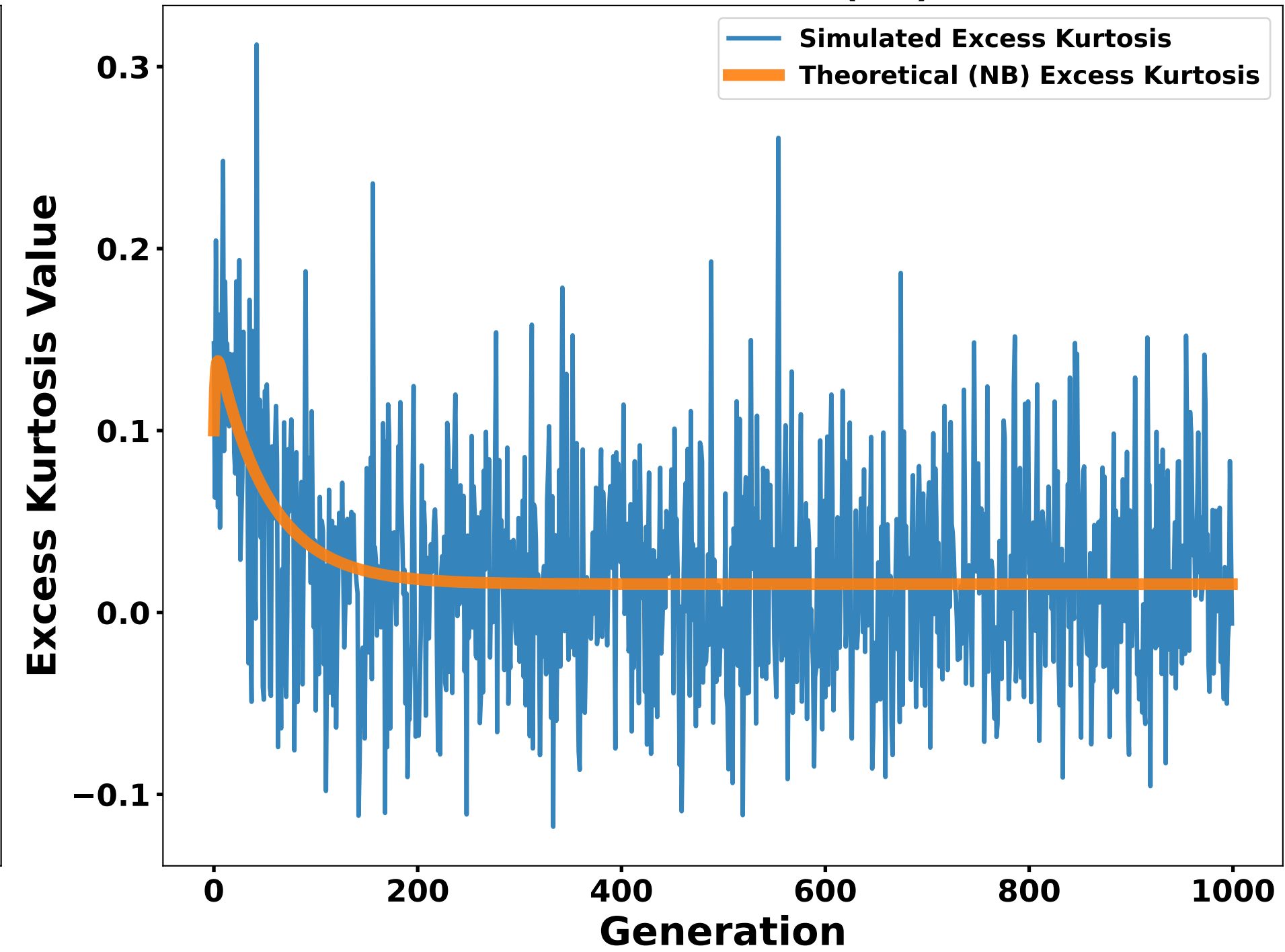
Excess Kurtosis (NB)
