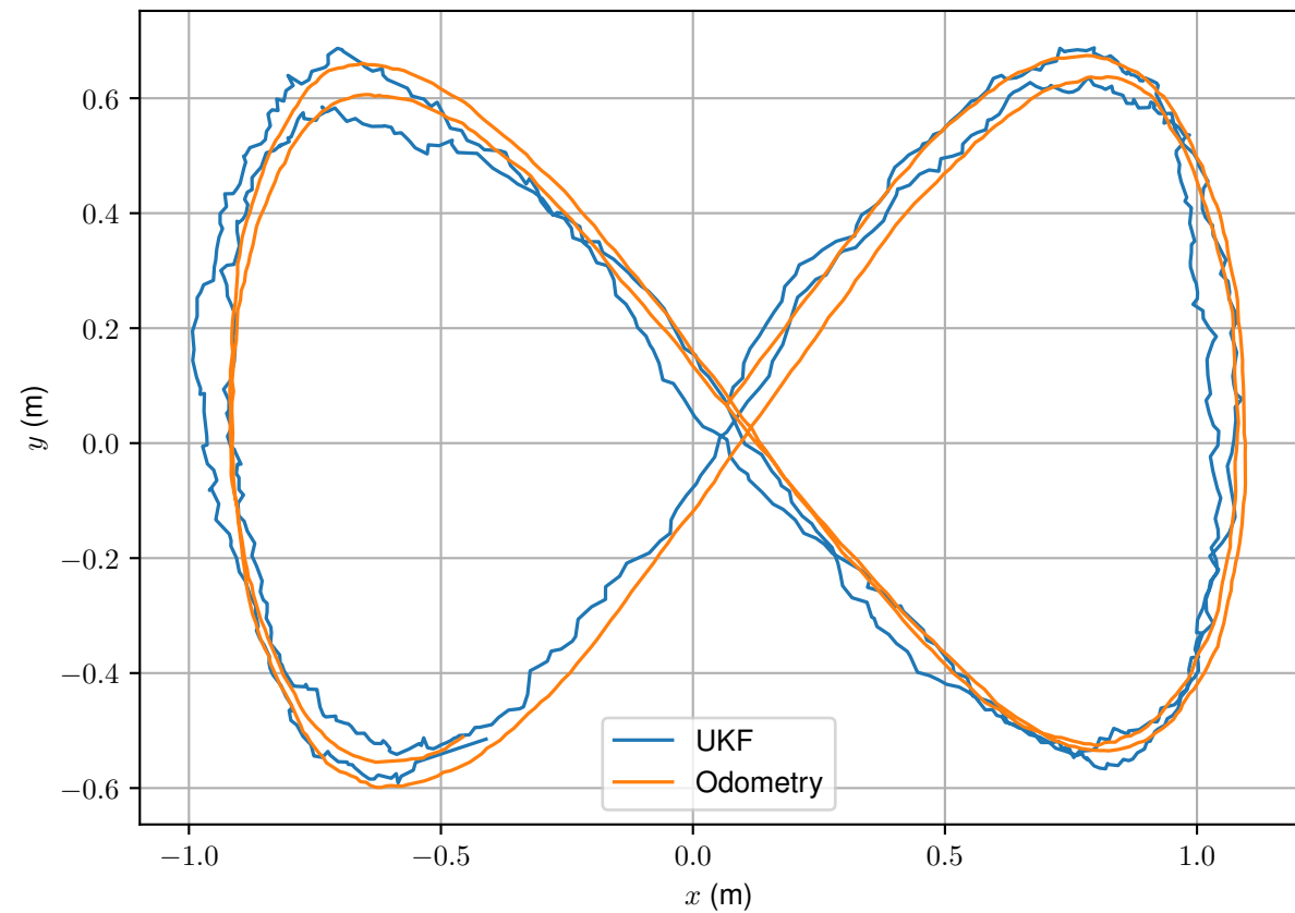
Vehicle Motion Visualization at \sigma^2 = 0.01
