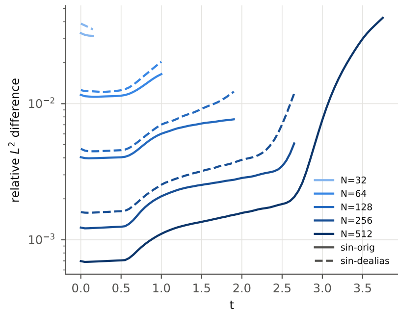
a = 0.5 : difference from the sin-dealias N=512 solution
