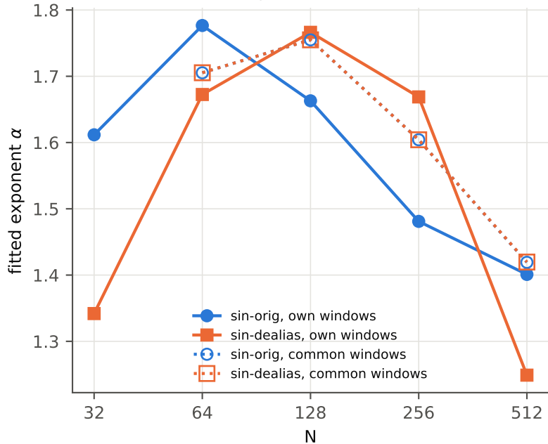
own windows: differ because the stopping times differ common windows: overlap of both schemes' windows at each N
