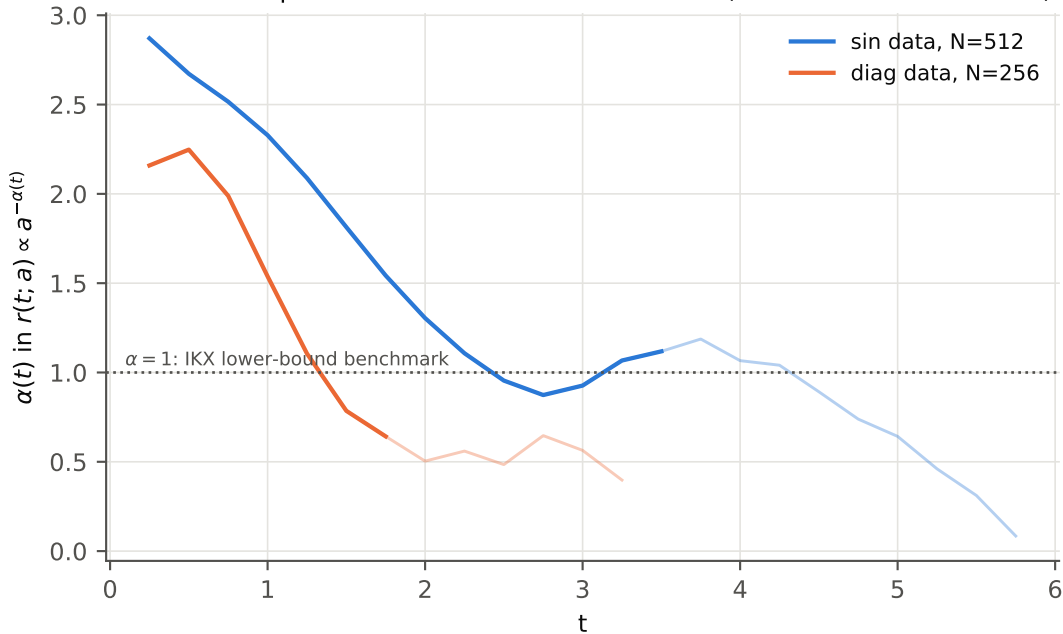
fixed-time exponent for two initial-data families (faded: not all a resolved)
