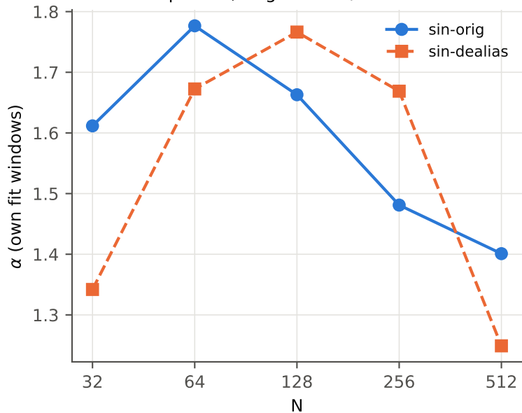
fitted exponent, original vs 2/3-rule dealiased
