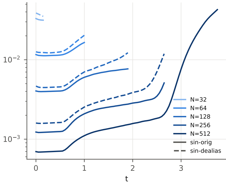
a = 0.5 : L^2 error vs reference sin-dealias:512
