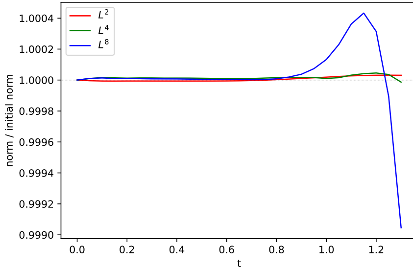
Figure 4: L^p norms normalised to their initial values for a = 0.5 . All three norms should stay \approx 1 ; a sustained drift triggers the resolution-check event that stops the integration.
