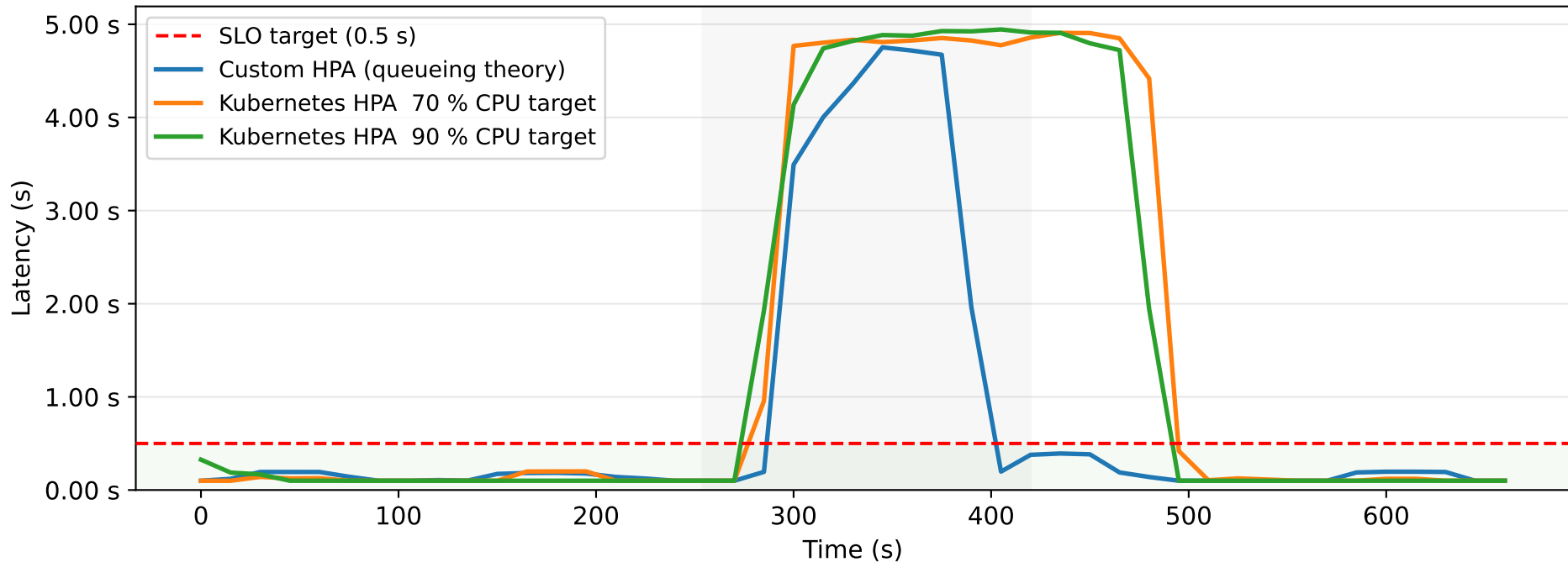
p99 Server-Side Inference Latency
