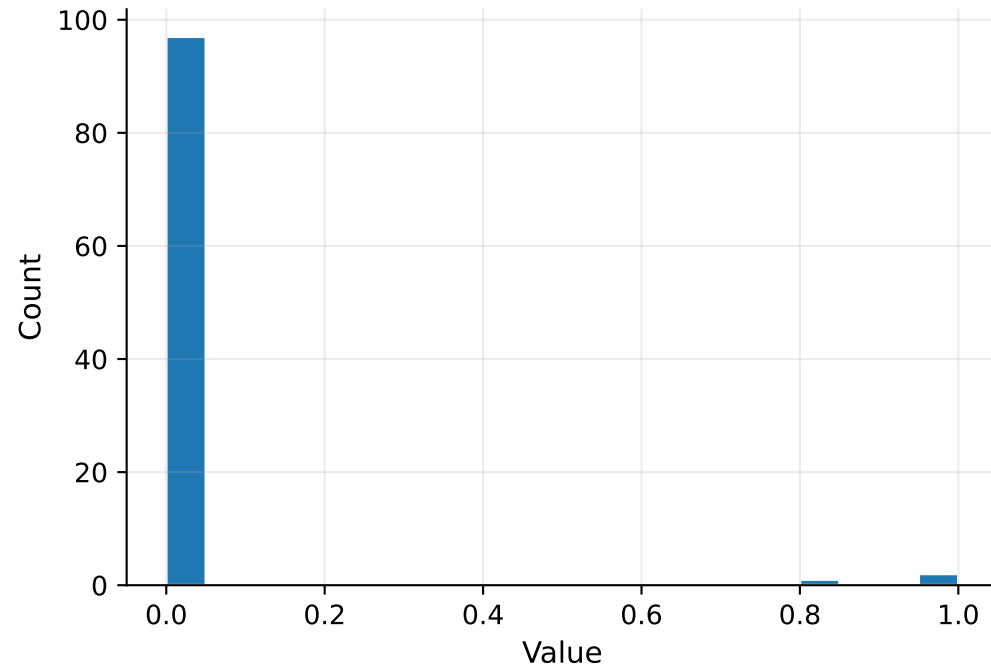
exp_07_tms_5_2_4layer_untied_rep1 | hidden_layers.1 lower-CI histogram
