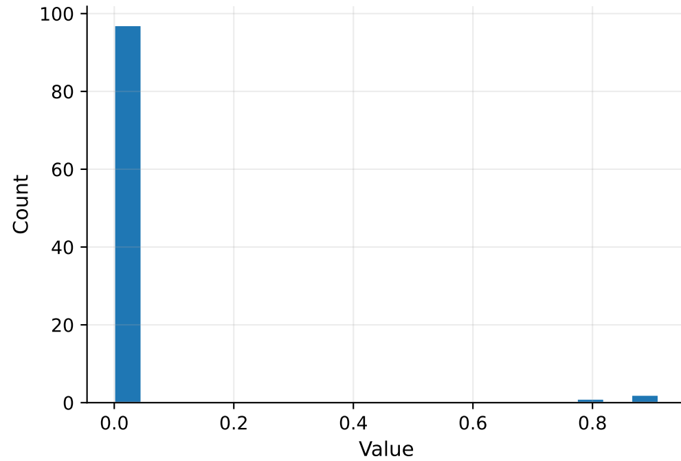
exp_07_tms_5_2_5layer_untied_rep1 | hidden_layers.1 lower-CI histogram
