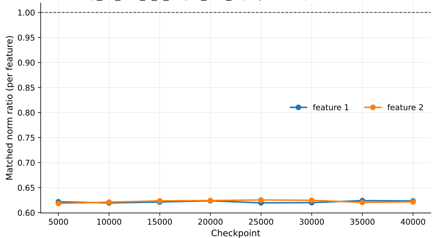
exp_07_tms_5_2_2layer_tied_rep1 | linear2 per-feature ML2R
