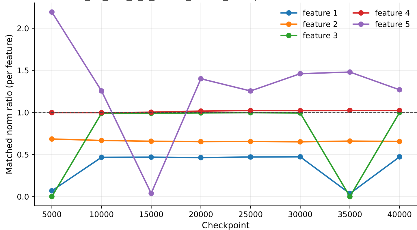
exp_07_tms_5_2_2layer_untied_rep1 | linear1 per-feature ML2R
