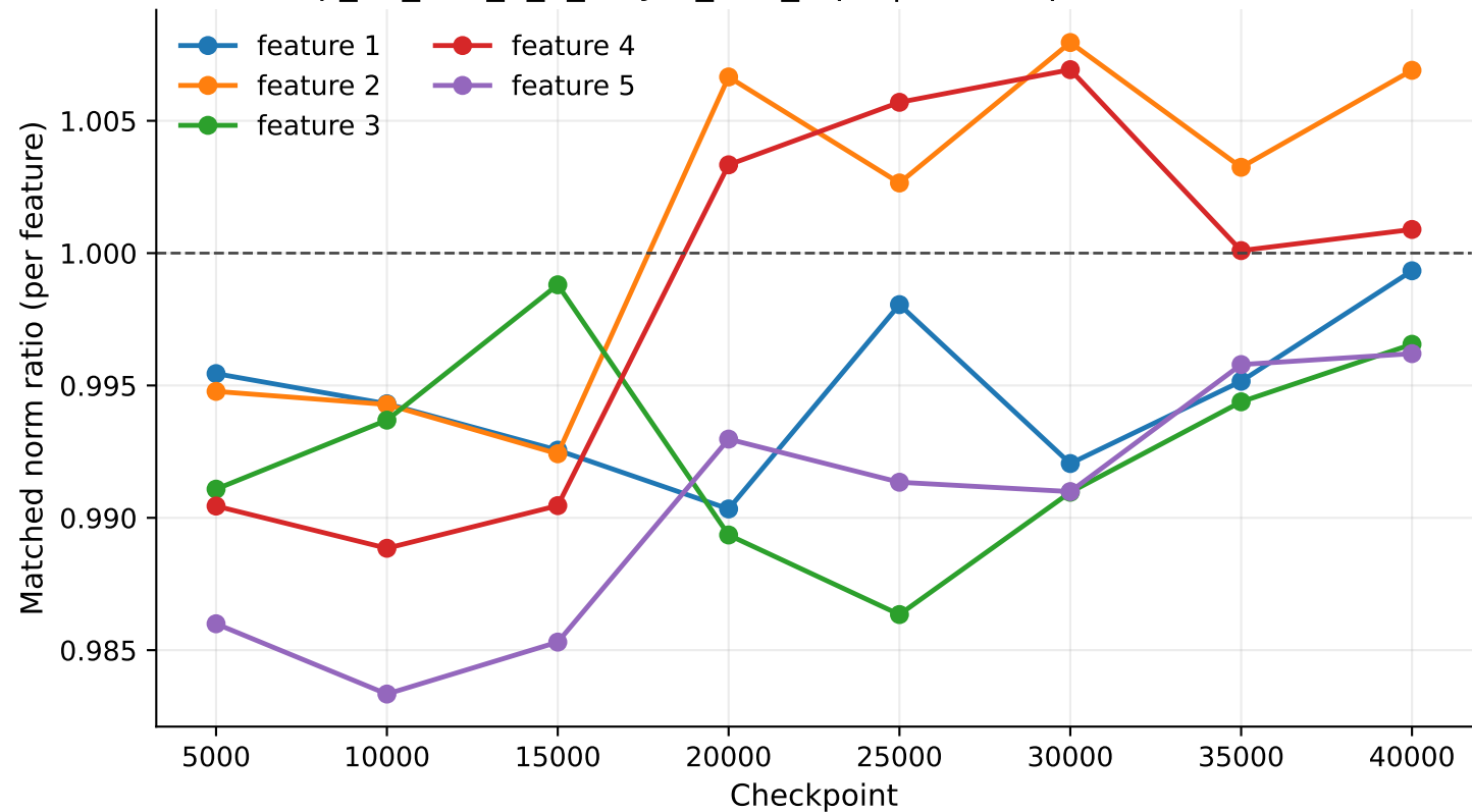
exp_07_tms_5_2_3layer_tied_rep1 | linear1 per-feature ML2R
