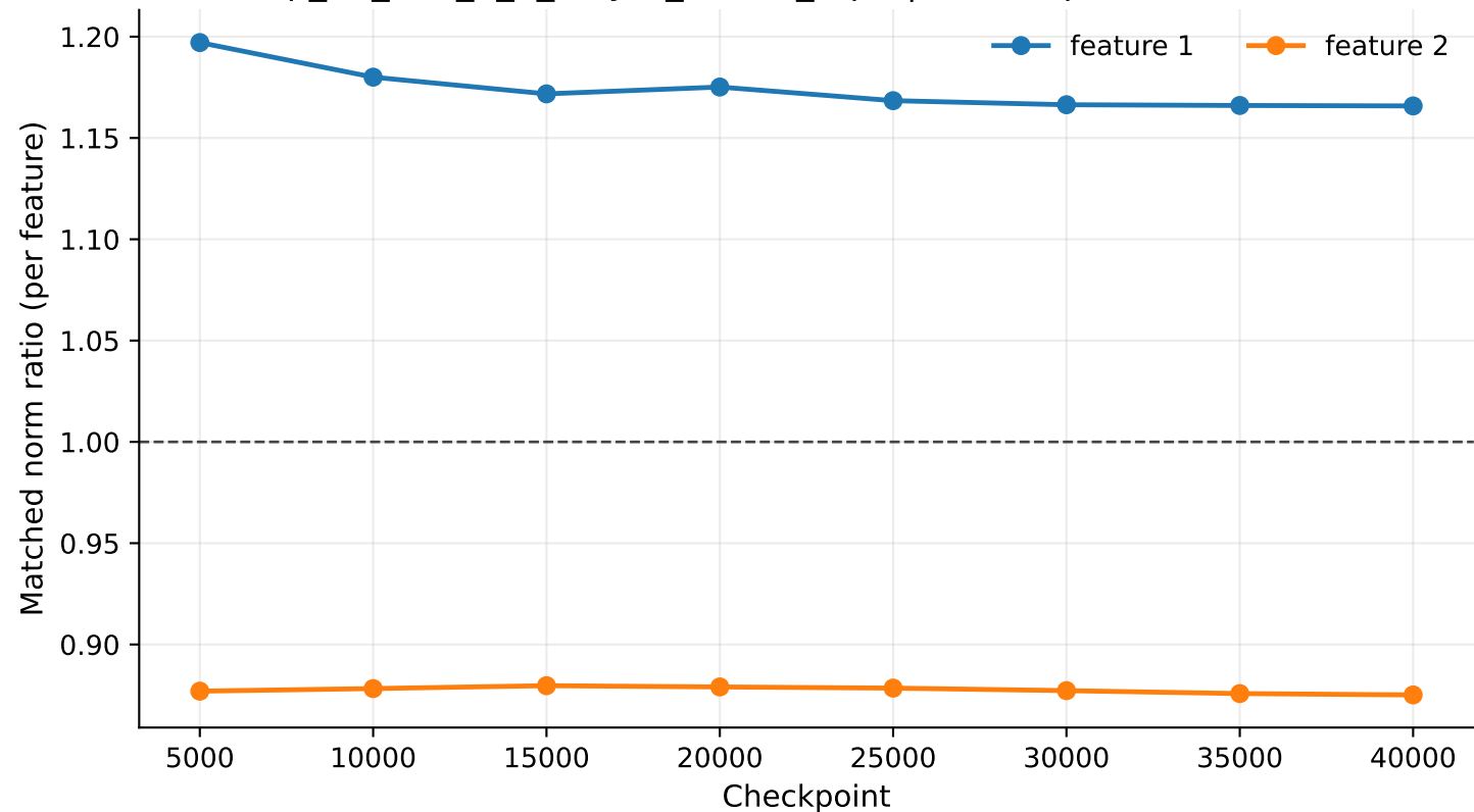
exp_07_tms_5_2_3layer_untied_rep1 | linear2 per-feature ML2R
