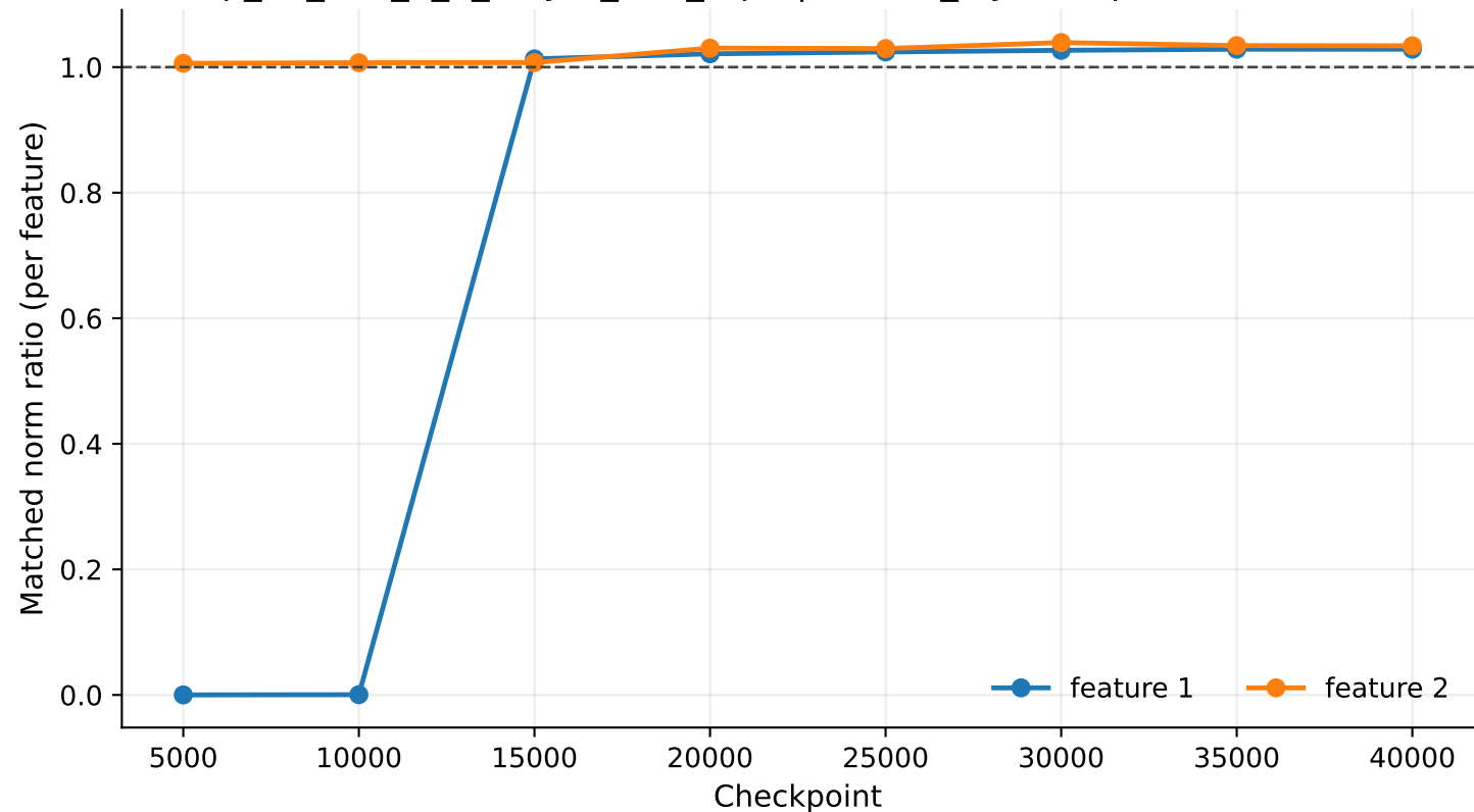
exp_07_tms_5_2_4layer_tied_rep1 | hidden_layers.1 per-feature ML2R
