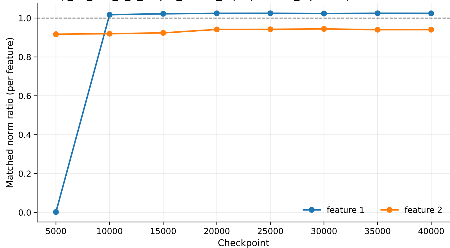
exp_07_tms_5_2_4layer_untied_rep1 | hidden_layers.0 per-feature ML2R
