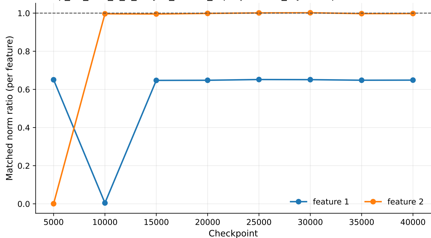
exp_07_tms_5_2_4layer_untied_rep1 | hidden_layers.1 per-feature ML2R
