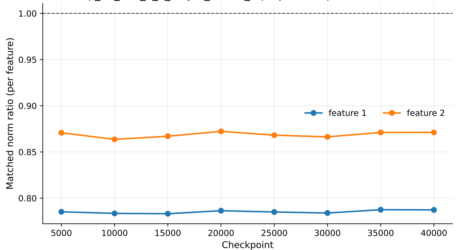
exp_07_tms_5_2_4layer_untied_rep1 | linear2 per-feature ML2R
