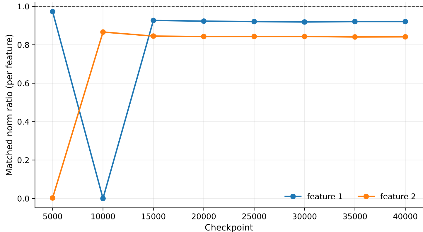
exp_07_tms_5_2_5layer_tied_rep1 | hidden_layers.1 per-feature ML2R
