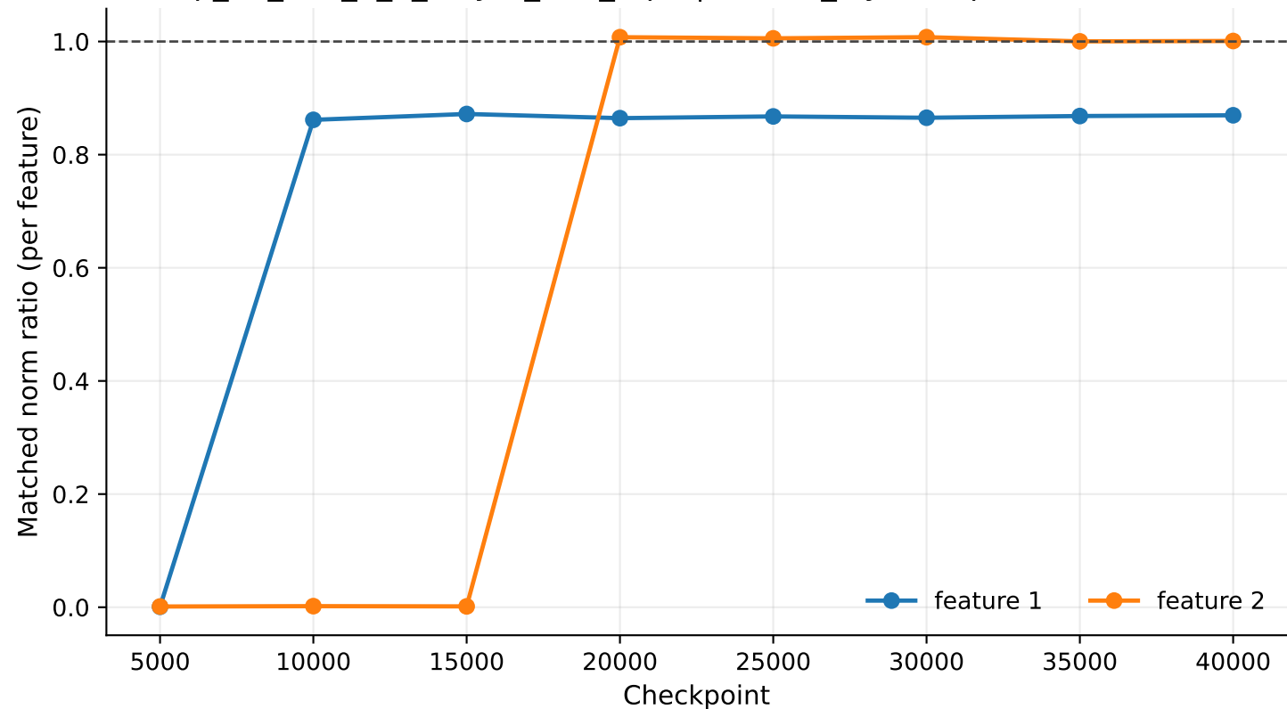
exp_07_tms_5_2_5layer_tied_rep1 | hidden_layers.2 per-feature ML2R
