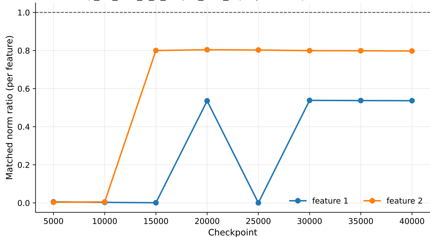
exp_07_tms_5_2_5layer_tied_rep1 | linear2 per-feature ML2R
