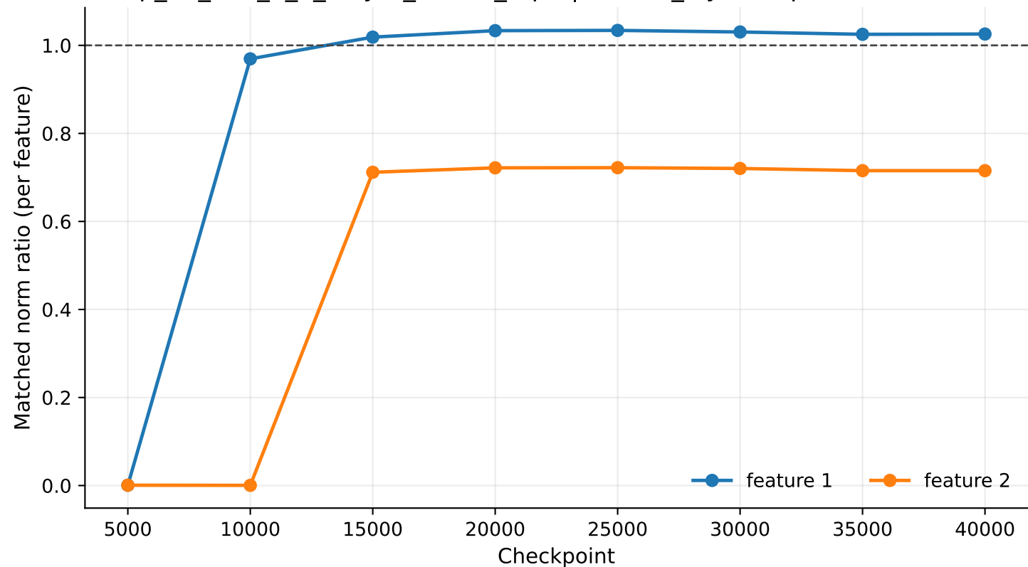
exp_07_tms_5_2_5layer_untied_rep1 | hidden_layers.0 per-feature ML2R
