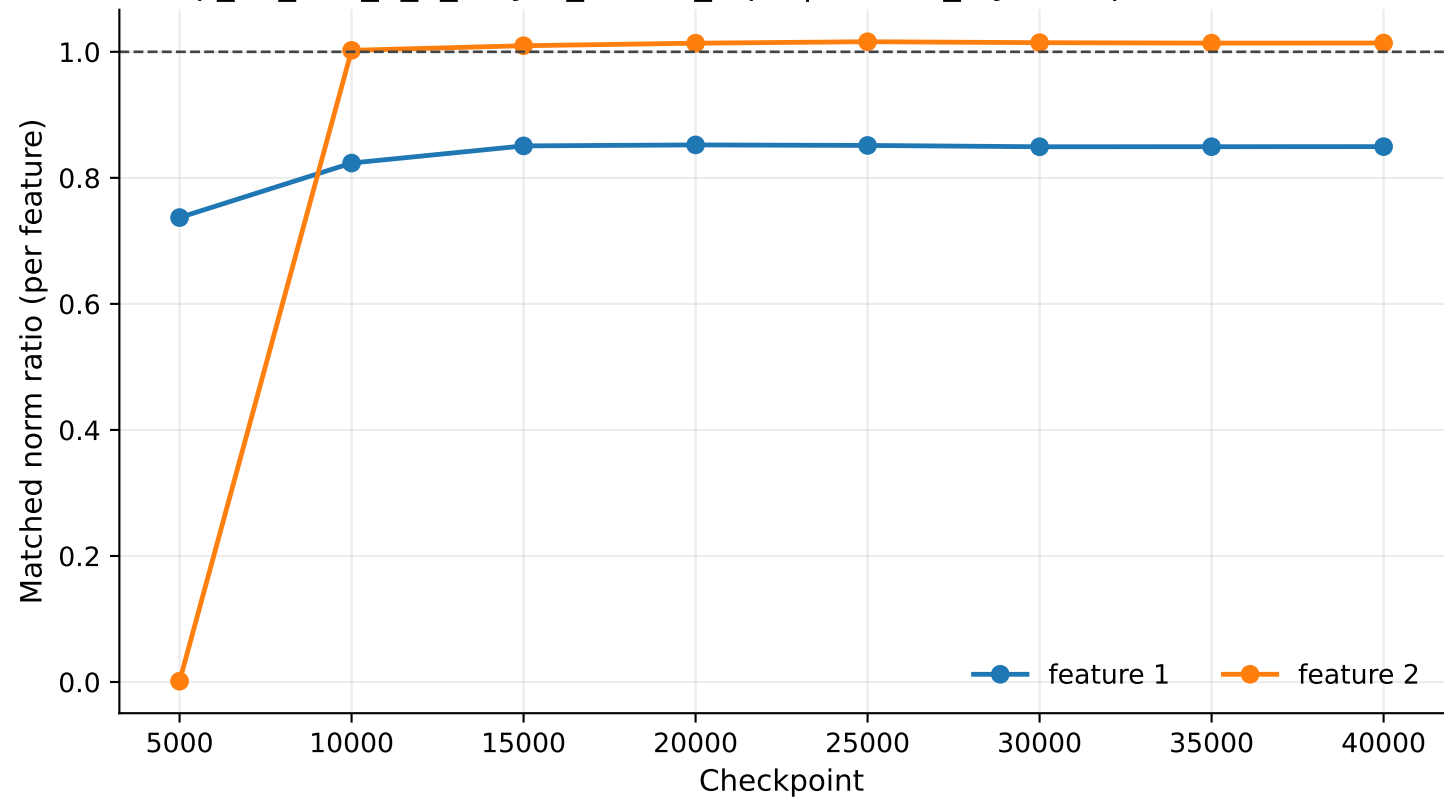
exp_07_tms_5_2_5layer_untied_rep1 | hidden_layers.2 per-feature ML2R
